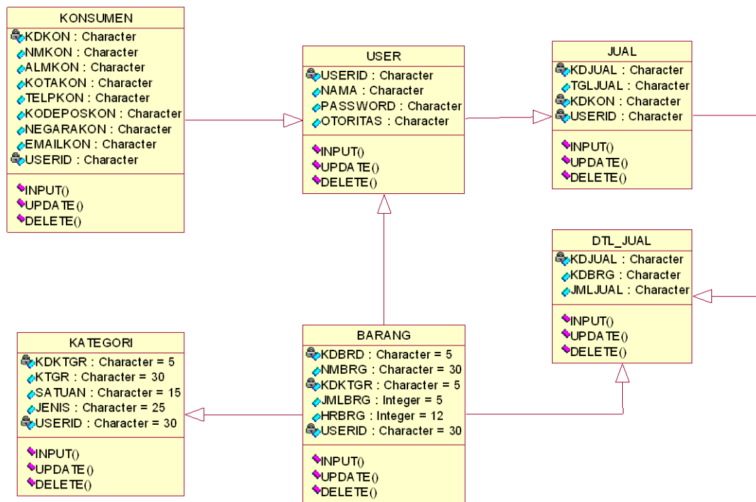
Gambar 3 : Class Diagram
