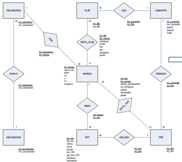
Gambar 5: Entity-Relationship Diagram
