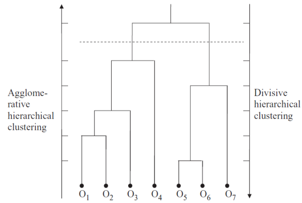
Gambar Hierarchical clustering sumber (Xu & Wunsch, 2009)
