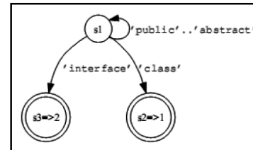
Gambar 3. Cyclic DFA
