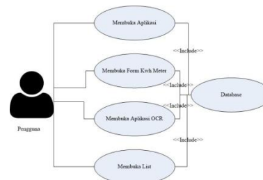
Gambar 19. Use Case Diagram
