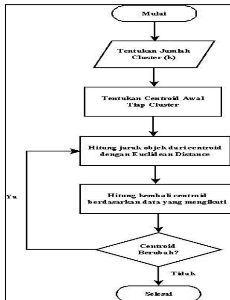
Gambar 3. Flowchart Algoritma K-Means
