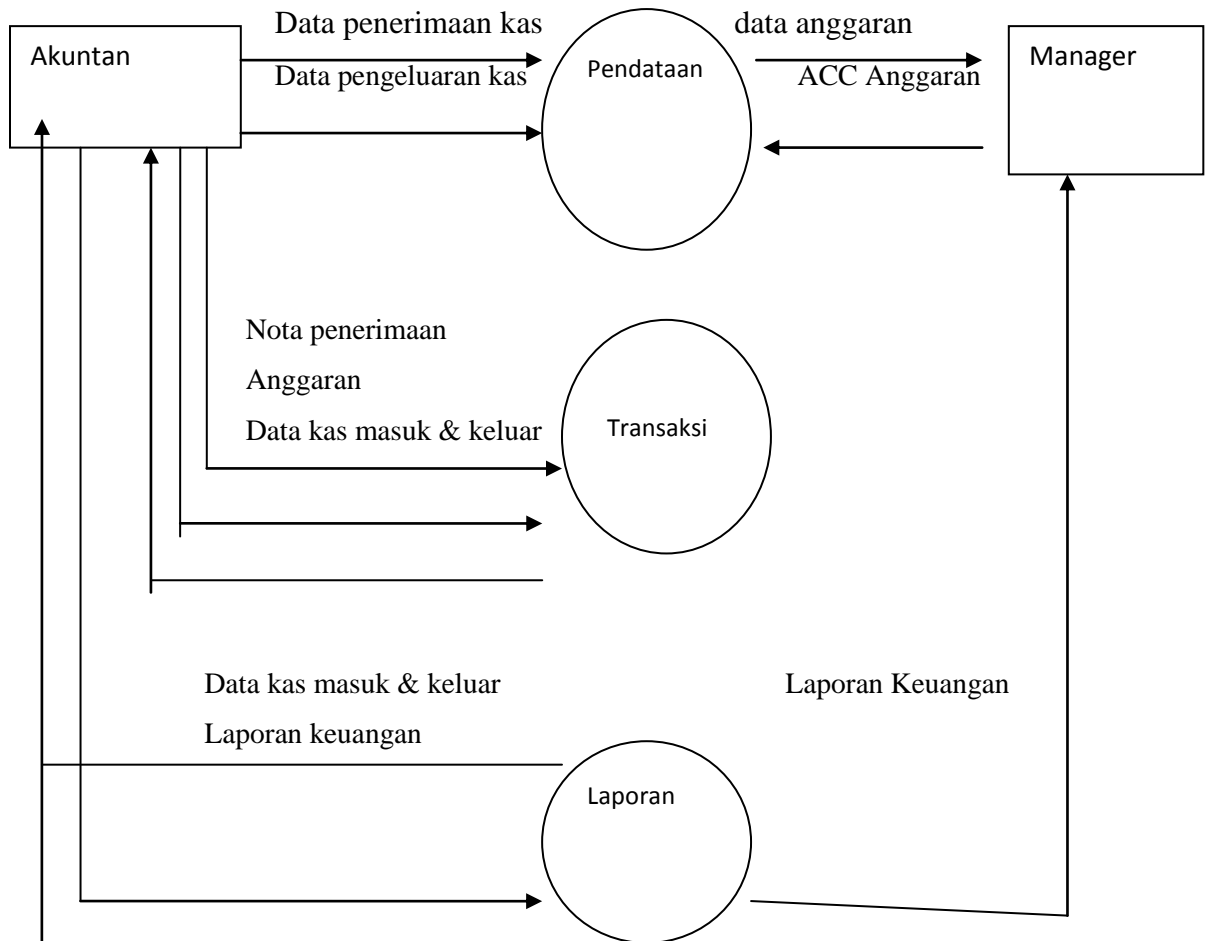
Gambar 4.4 DFD Level 1
