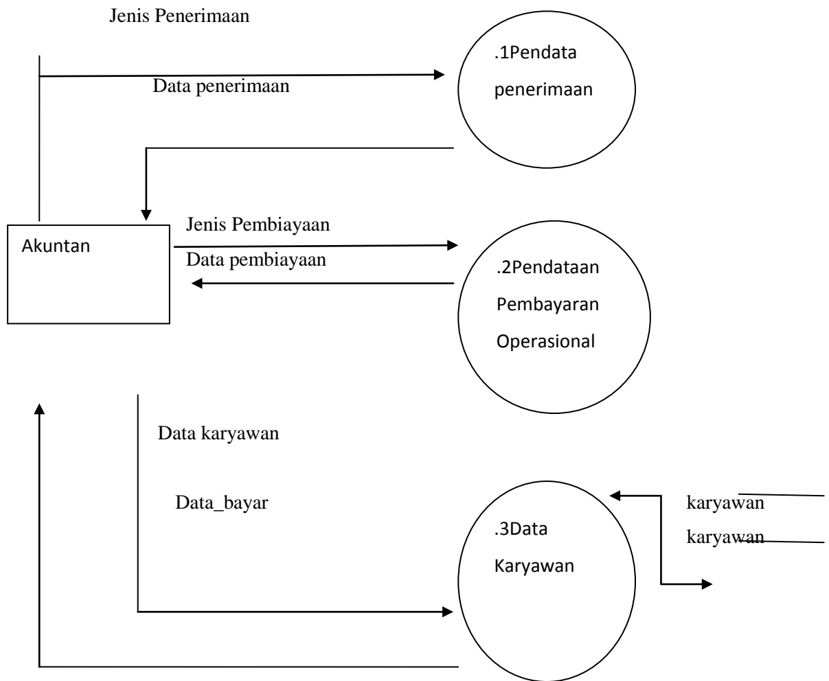
Gambar 4.4 DFD Level 1 Proses Pendataan
